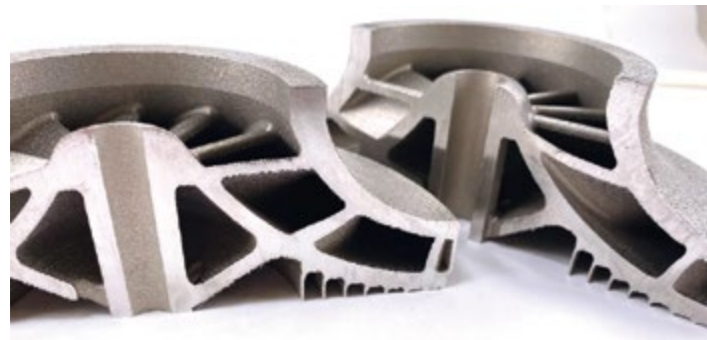
Figure 2: Cross section of a support-free impeller
