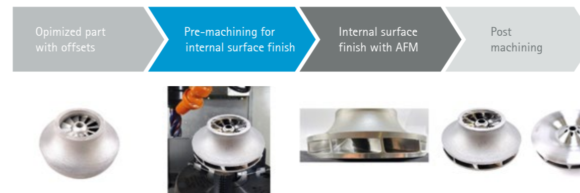
Figure 15: Manufacturing workflow for closed impellers
